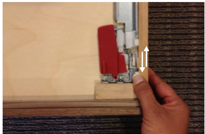
Figure 3. Level the drawer slides
