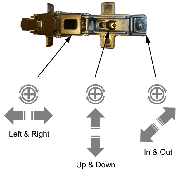
Figure 4. Adjust the door(s) by turning the screws on the hinge.
